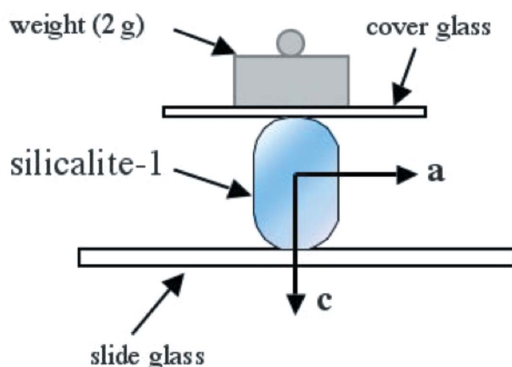
Figure 4 Pressing treatment for the phase transition from the monoclinic twin to the orthorhombic single silicalite-1 crystal.
