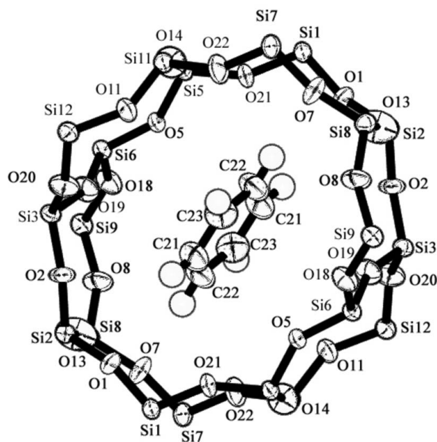
Figure 11 Ben2 and the straight channel framework in the benzene7.2-silicalite-1 structure along the b axis.
