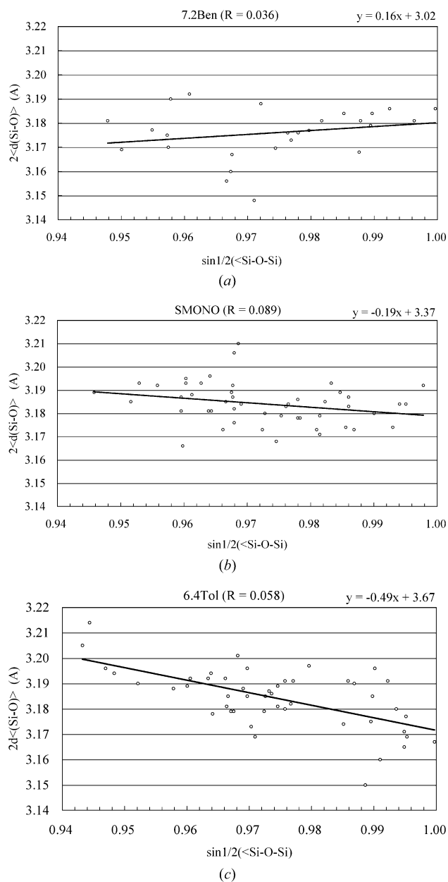
Figure 5 Scatter diagram of \langle d(\text{Si}-\text{O}) \rangle , plotted as a function of \sin 1/2(\angle \text{SiOSi}) in (a) 7.2Ben, (b) SMONO and (c) 6.4Tol.
