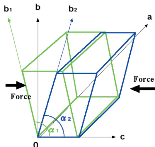
Figure 3 Model of a monoclinic twin silicalite-1 crystal and definitions of \alpha_1 and \alpha_2 .
