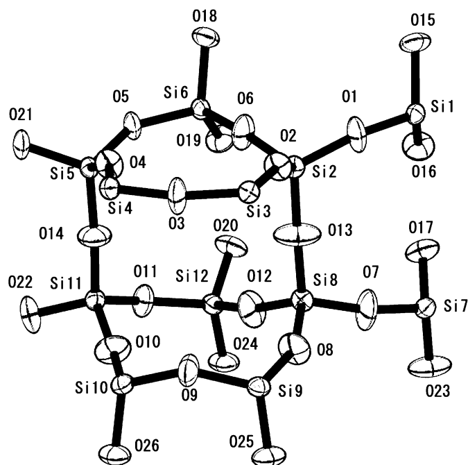
Figure 6 Asymmetric unit of silicalite-1 using the space group Pnma .
