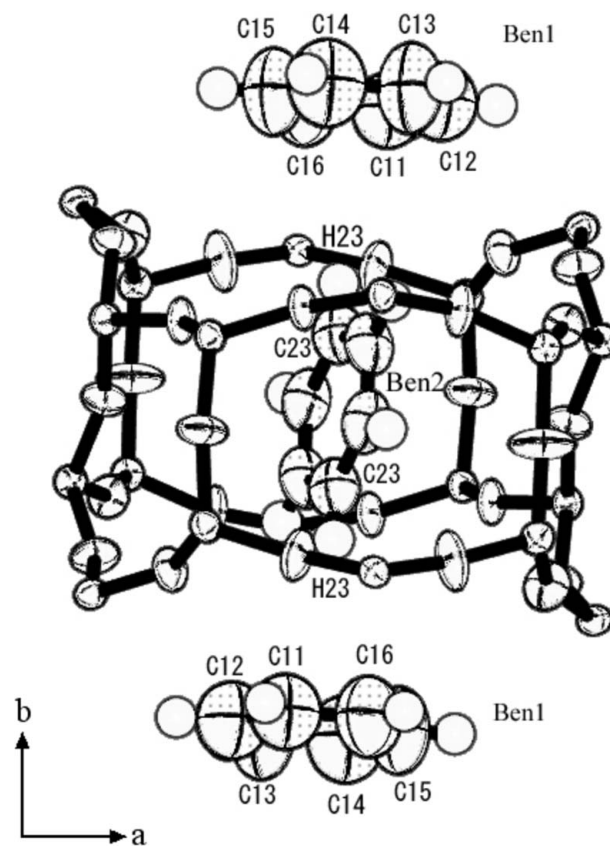
Figure 9 Ben1, Ben2 and the straight channel framework in the benzene7.2-silicalite-1 structure.
