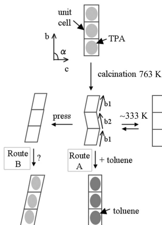
Figure 2 Model of the phase transitions of MFI zeolite.
