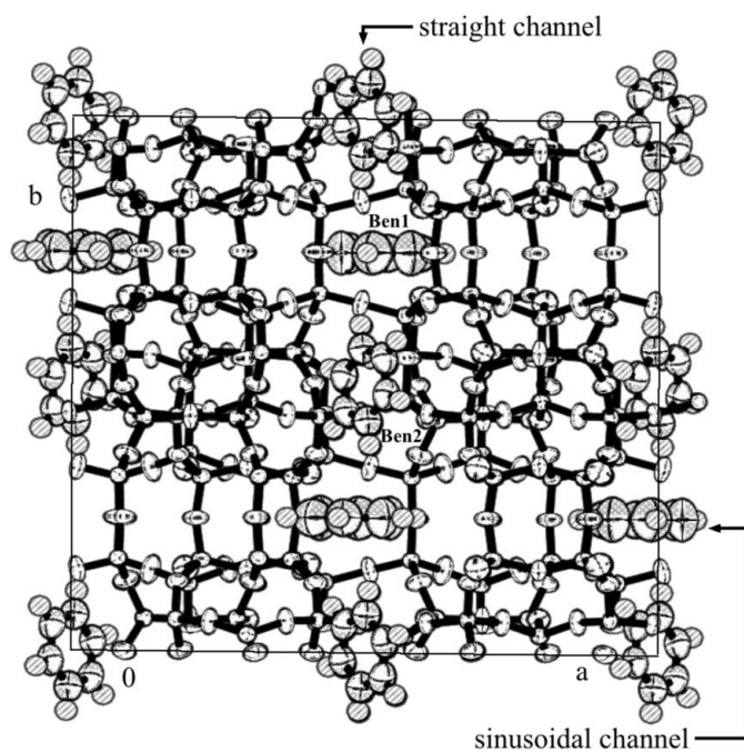
Figure 7 Packing view of benzene7.2-silicalite-1 along the c axis.
