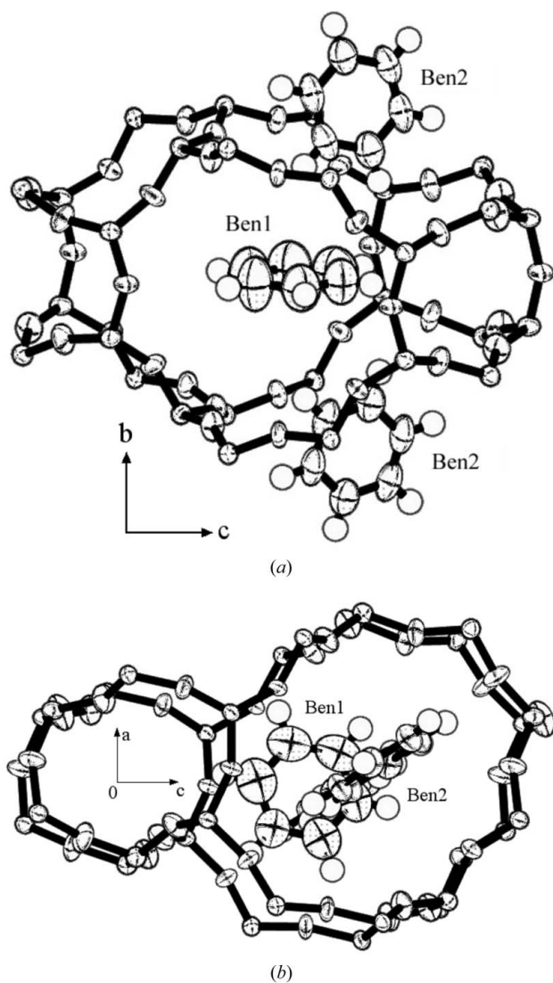
Figure 10 Ben1, Ben2 and the intersection cage in the benzene7.2-silicalite-1 structure: ( a ) along the a axis and ( b ) along the b axis.
