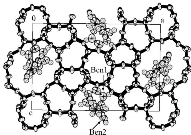
Figure 8 Packing view of benzene7.2-silicalite-1 along the b axis.
