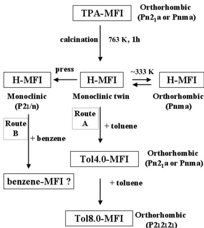
Figure 1 Phase transitions of MFI zeolite.
